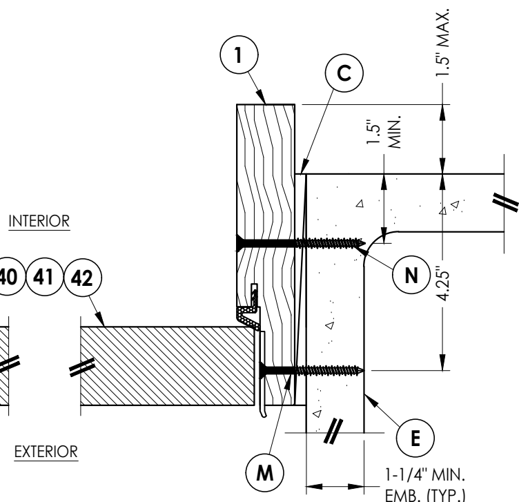
6 HORIZONTAL CROSS SECTION Shown Direct to Masonry Outswing only w/ 6-9/16" jamb
