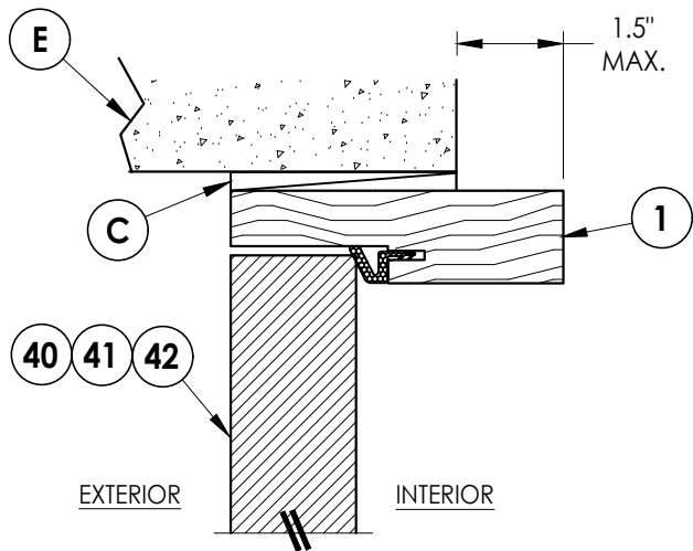
1 VERTICAL CROSS SECTION Shown Direct to Masonry Outswing only w/ 4-9/16" jamb
