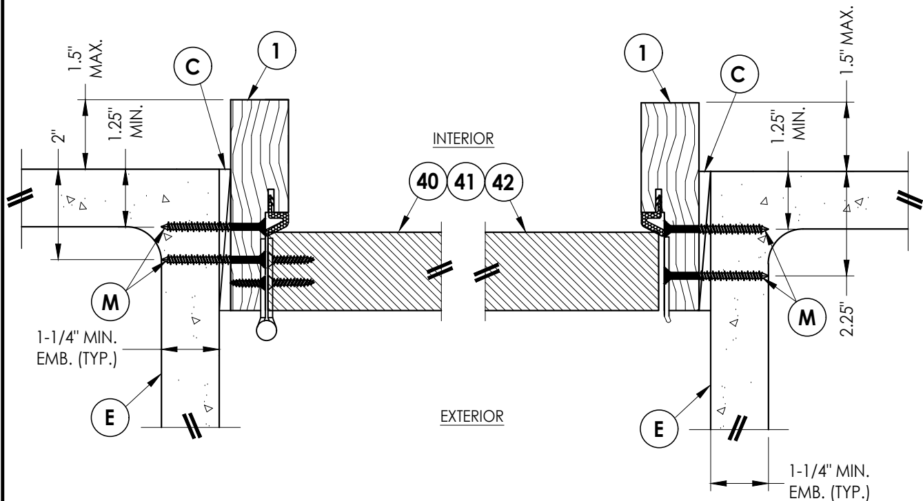
2 HORIZONTAL CROSS SECTION Shown Direct to Masonry Outswing only w/ 4-9/16" jamb
