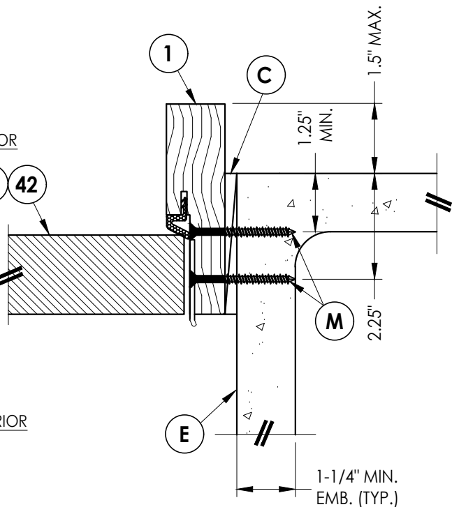
3 HORIZONTAL CROSS SECTION Shown Direct to Masonry Outswing only w/ 4-9/16" jamb
