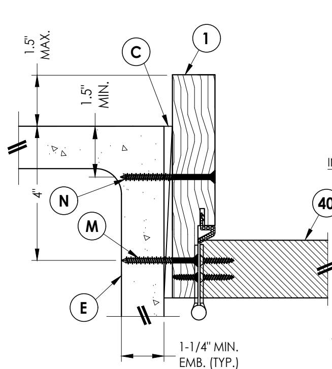
5 HORIZONTAL CROSS SECTION Shown Direct to Masonry Outswing only w/ 6-9/16" jamb
