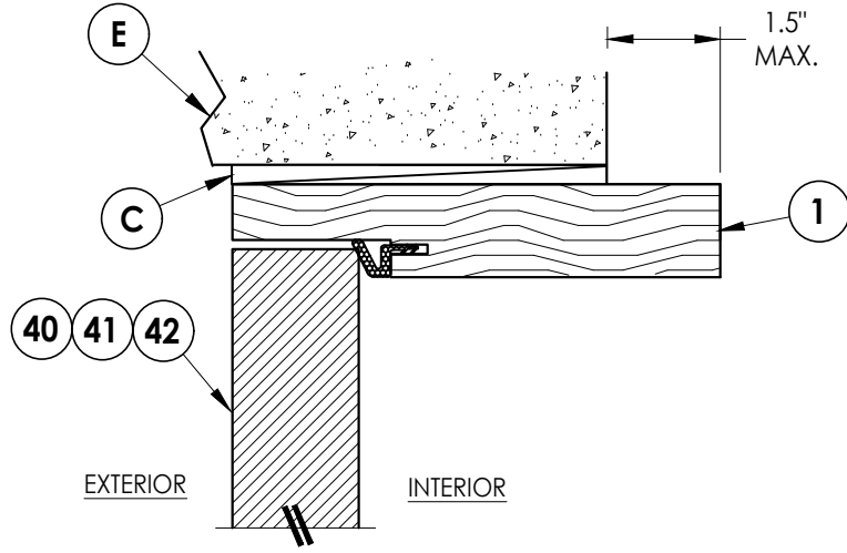
4 VERTICAL CROSS SECTION Shown Direct to Masonry Outswing only w/ 6-9/16" jamb
